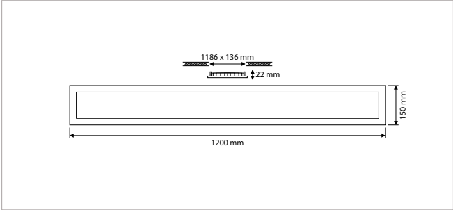
PRO-CEILING - RECTANGULAR - RECESSED - IP40 - 150 x 1200 x H 22 mm - CUTOUT 1186 x 136 mm - WHITE
