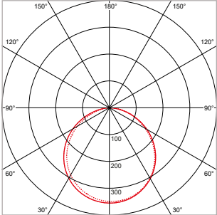
PRO-CEILING - RECTANGULAR - RECESSED - IP40 - 150 x 1200 x H 22 mm - CUTOUT 1186 x 136 mm - WHITE
